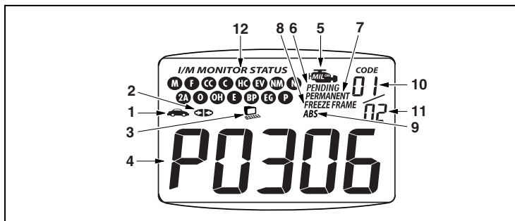
Figure 2. Display Functions
