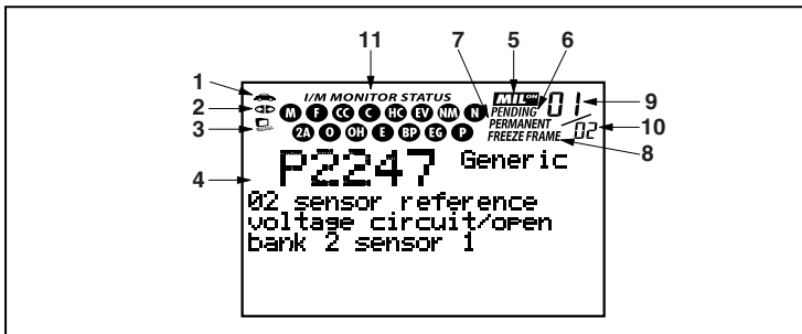
Figure 2. Display Functions
